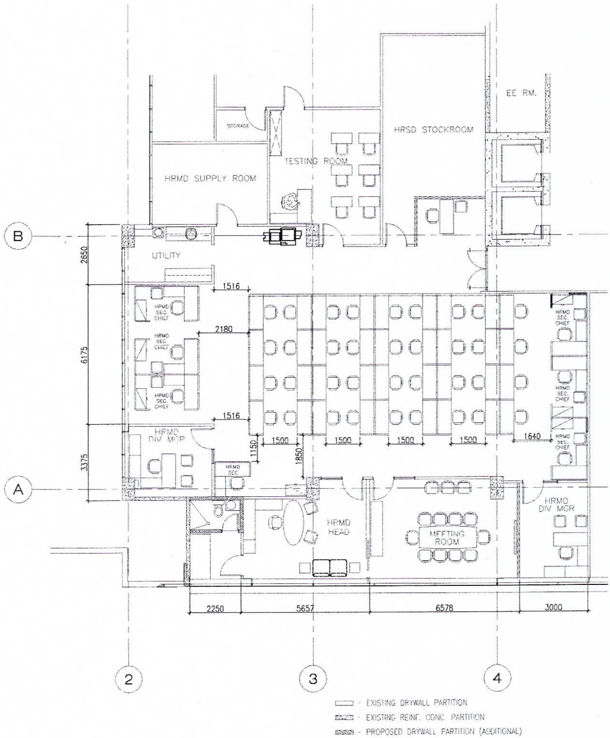
1 PROPOSED HRMD OFFICE LAYOUT (SCHEME-1) A-4 SCALE 1 : 100 MTS
