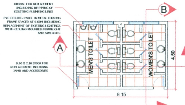
TYPICAL FLR. PLAN OF 1ST & 2ND FLR. CR
