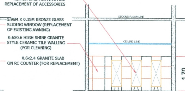
TYPICAL PLAN OF 1ST & 2ND FLR. C.R. SECTION "B"
