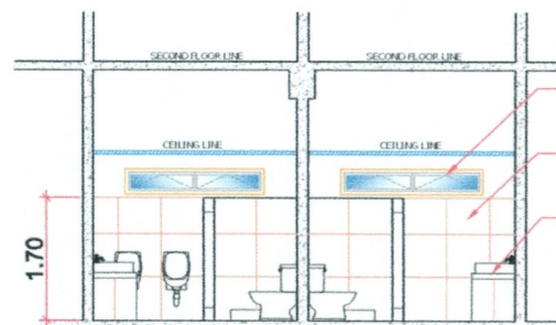
TYPICAL 1ST - 2ND FLR. PLAN SECTION "A"
