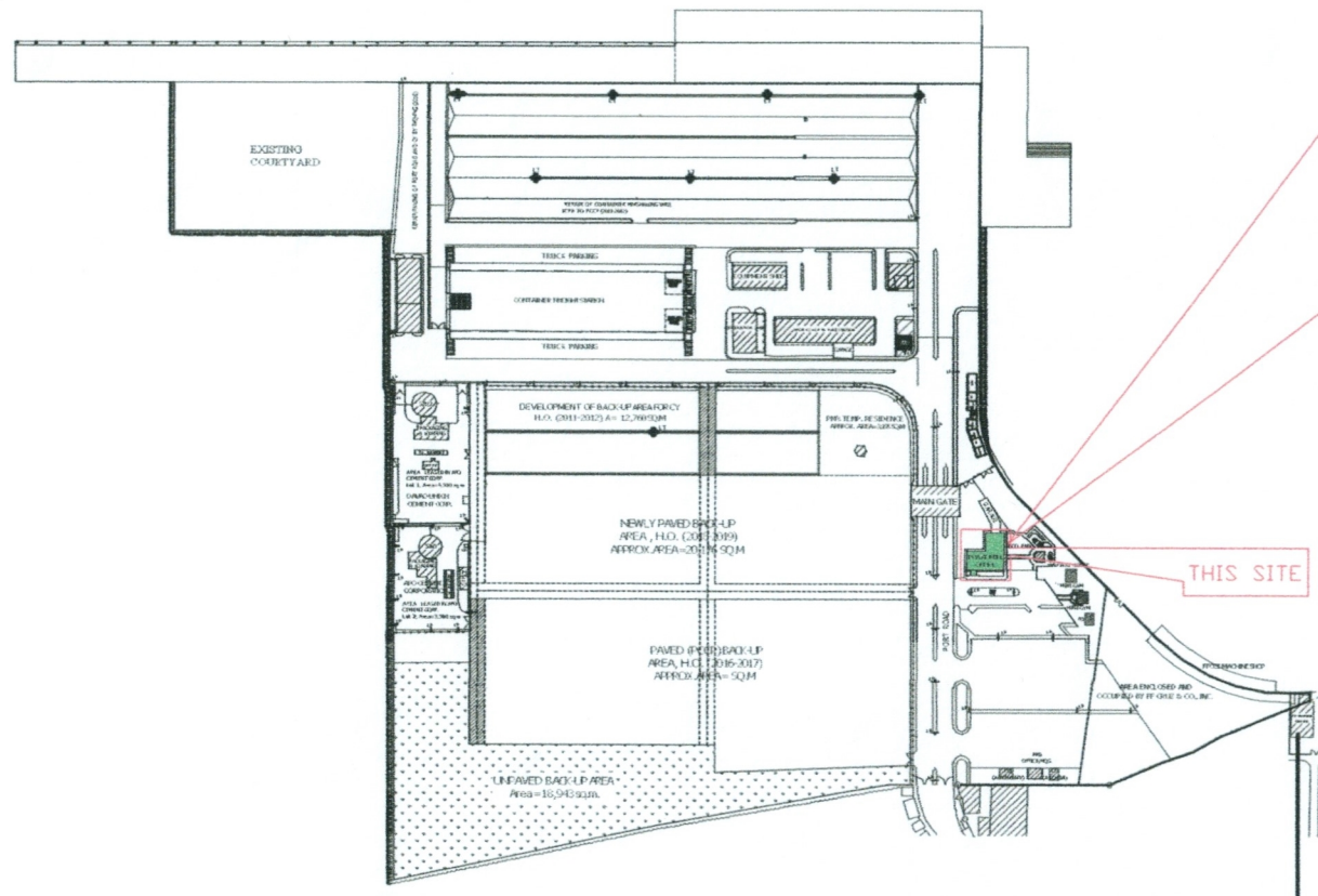
GENERAL PORT LAYOUT PLAN
