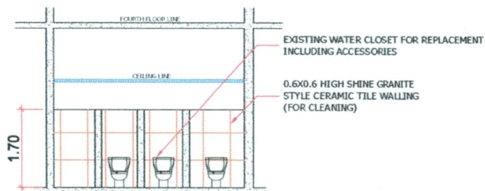
GROUND & SECOND FLOOR SECTION "B"
