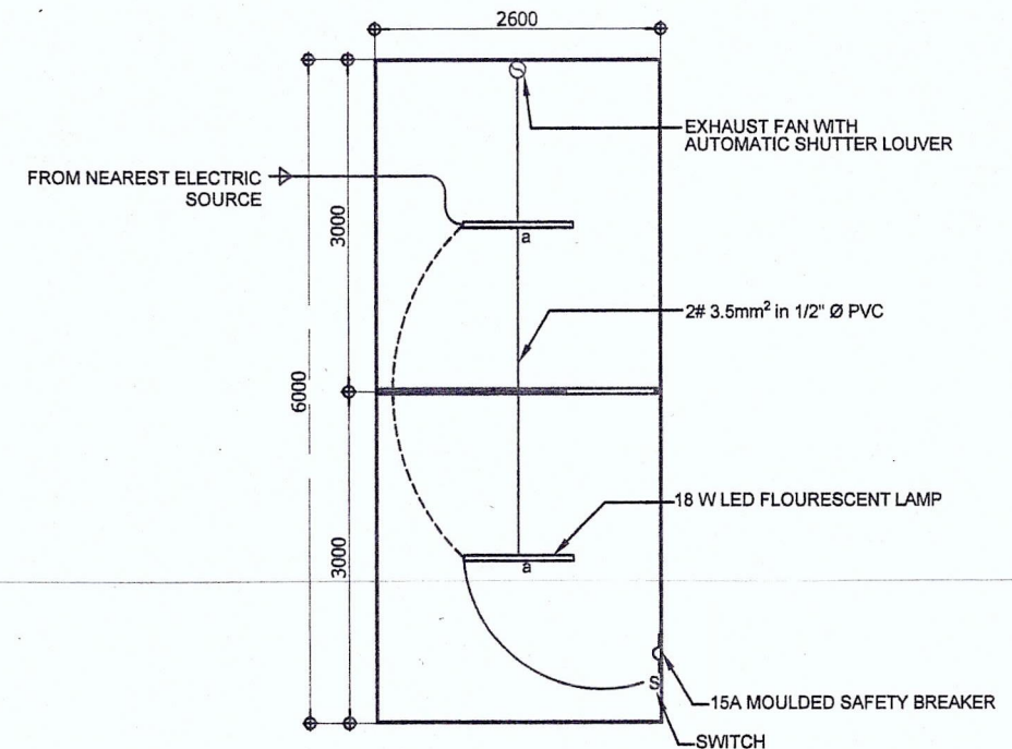
ELECTRICAL LAYOUT
