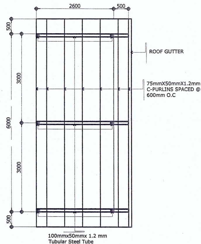
ROOF FRAMING PLAN
