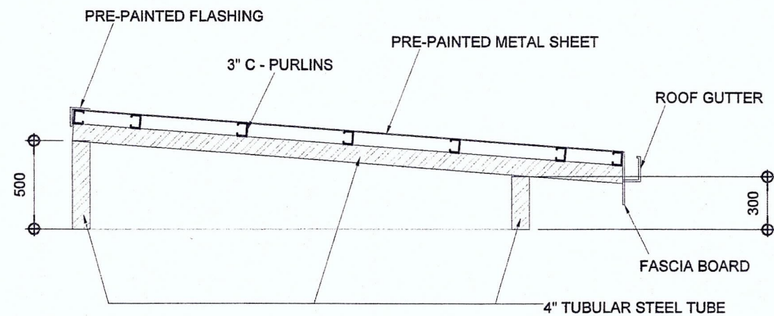
RAFTER DETAILS
