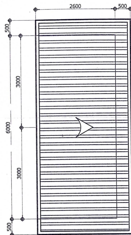
ROOF PLAN
