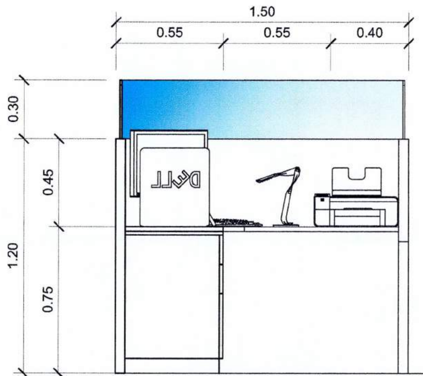
FRONT ELEV.
