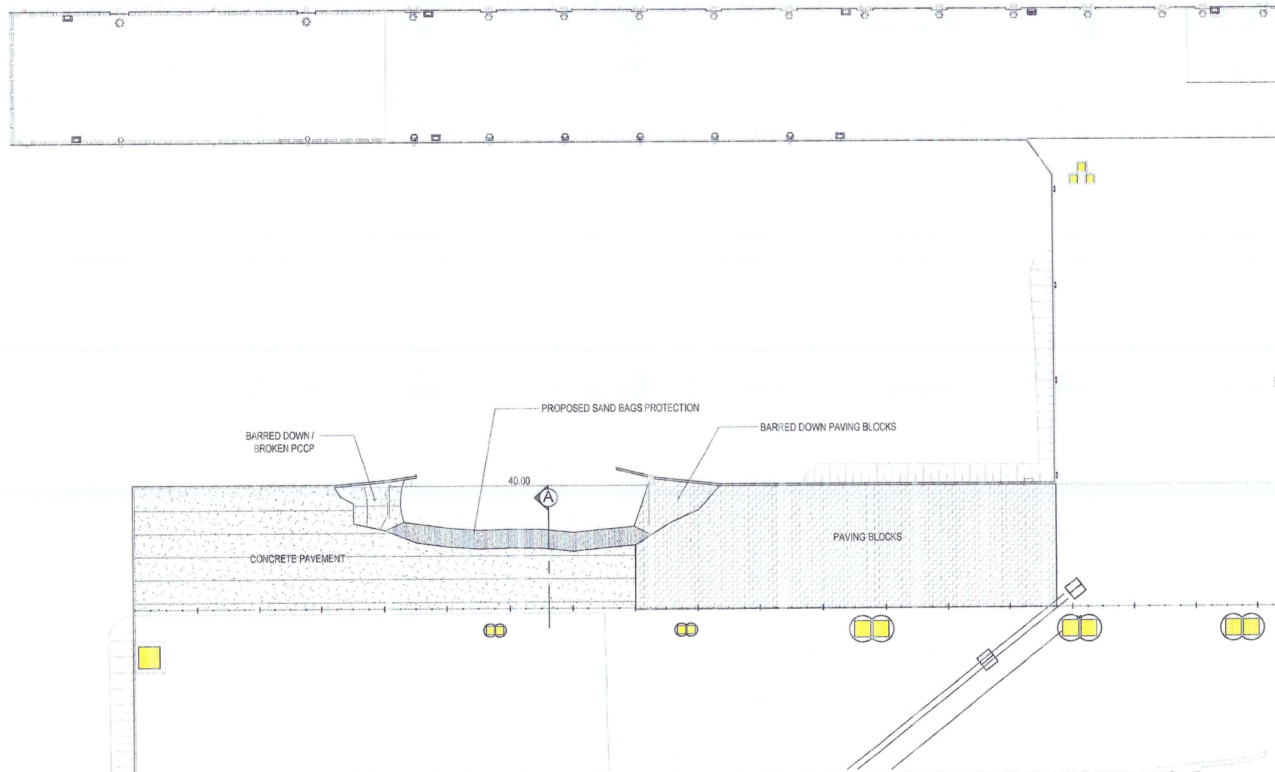
LAYOUT PLAN OF PROPOSED SANDBAGGING ALONG THE EDGE OF DAMAGED PAVEMENT AT BERTH NO. 2
