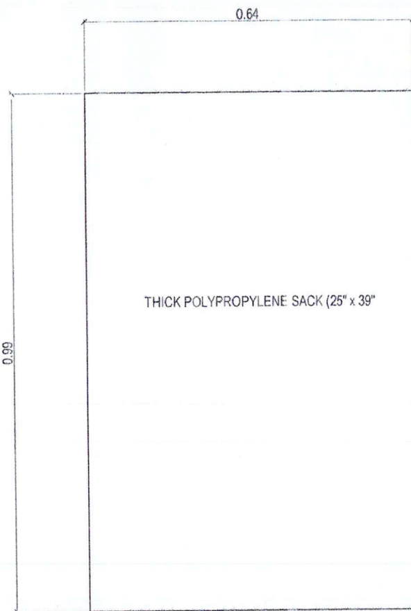
DIMENSION OF POLYPROPYLENE SACK SCALE 1:10 METERS
