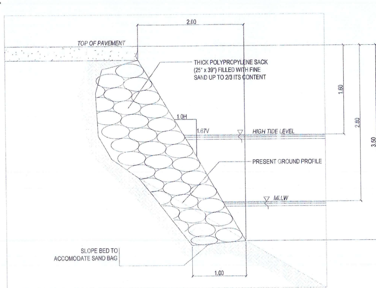
SECTION THRU "A" SCALE 1:40 METERS
