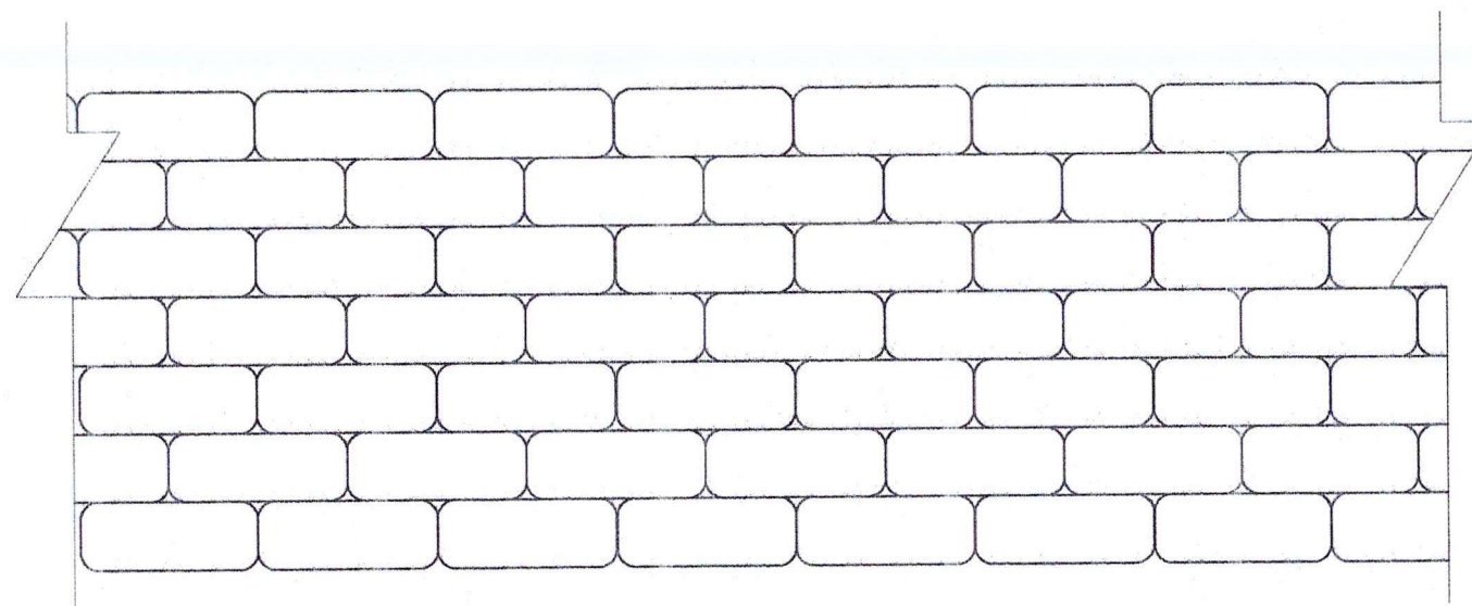
LAYING ARRANGEMENT OF SANDBAGS SCALE 1:30 METERS
